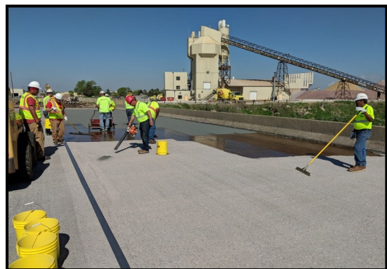
Crews placing a two-coat epoxy and chip seal on the Madison Street bridge. The chip seal gives the bridge surface a new wearing course to help with traction and preserve the life of the bridge deck.
